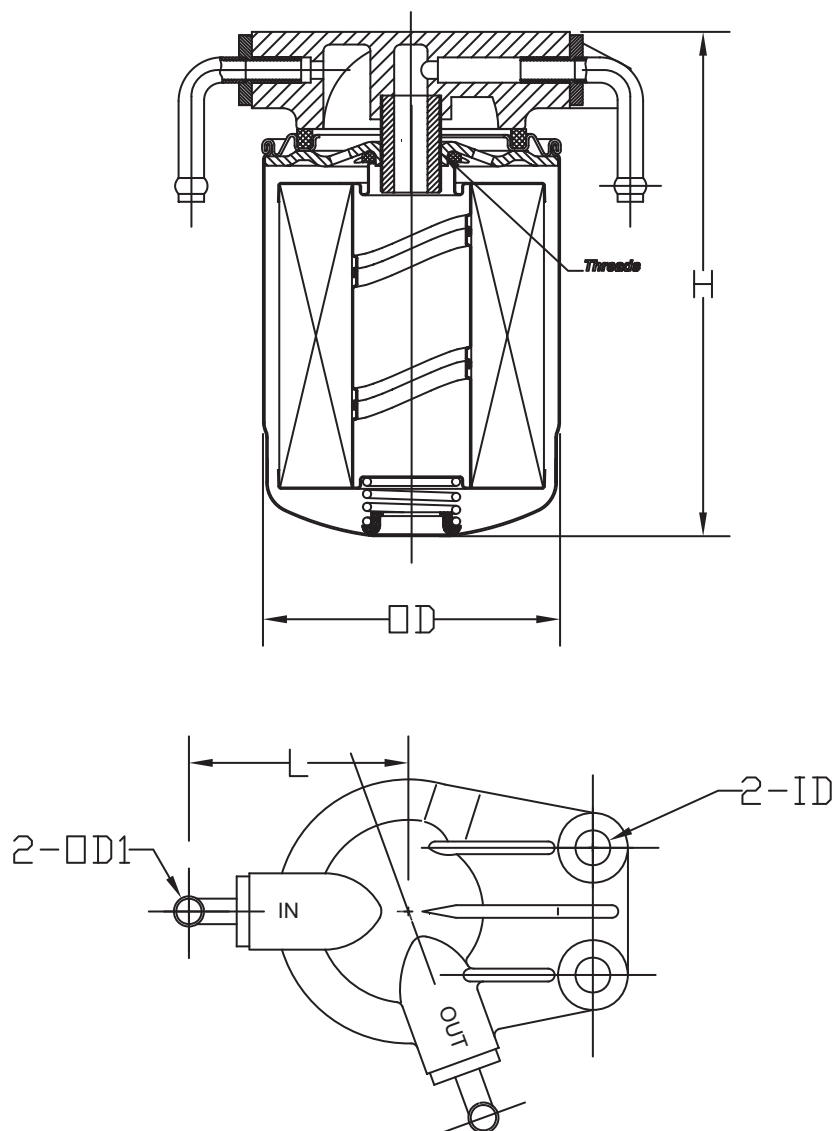
带底座燃油滤清器尺寸示意图 Fuel filter with head illustration
