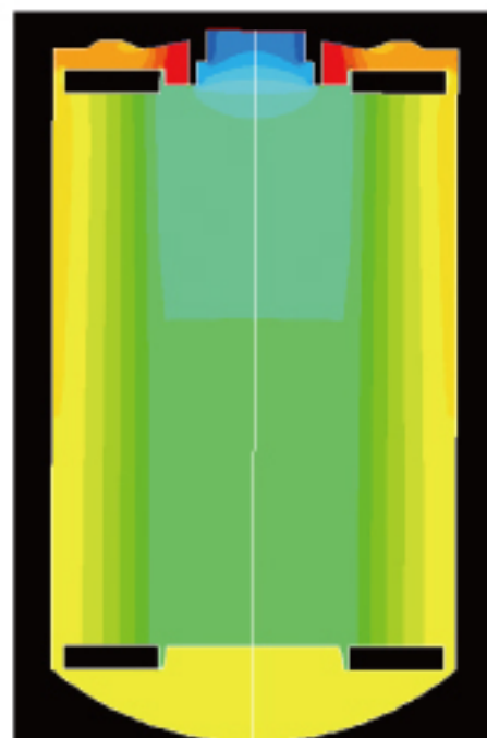
液体滤清器流场中各点静压分布 Static pressure distribution of flow field in liquid filters
