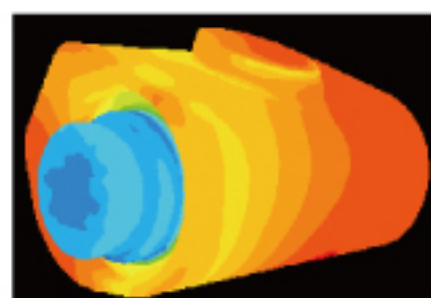
空滤进气系统的各点压力分布 Pressure distribution of air-intake system flow field
