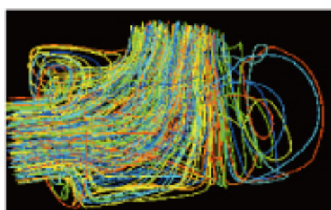
空滤进气系统的流线图，表明流场中各点的速度和方向 Flow path in flow field of air-intake system
